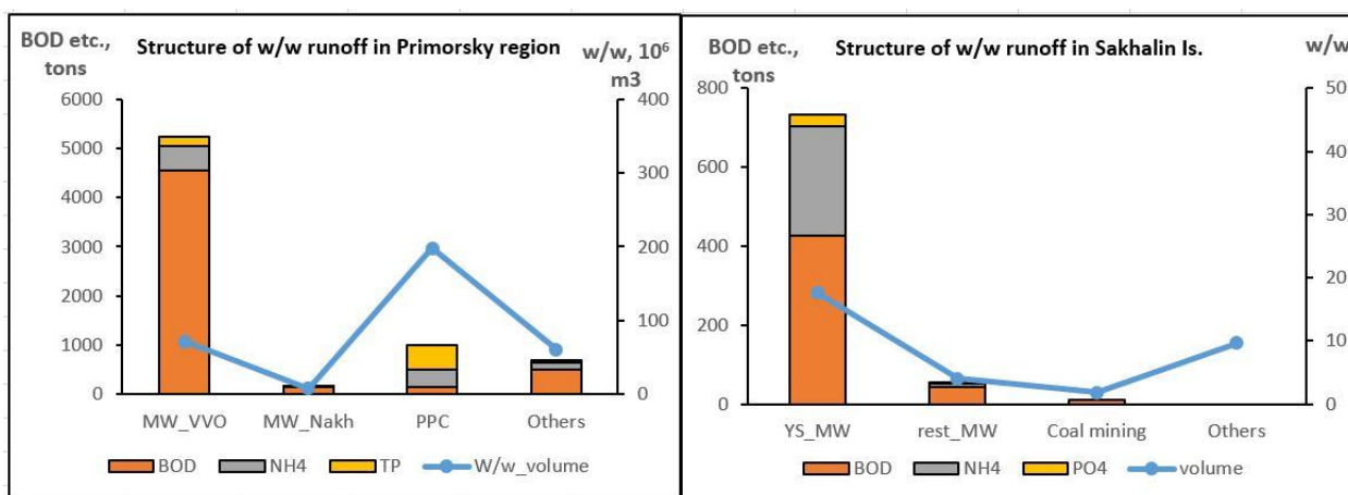
Figure 42. Major sources and structure of wastewaters inputs in Primorye and Sakhalin areas (Natural resources and Environmental protection of Primorye, 2017, Reports on ecological status and environmental protection in Sakhalin Oblast, 2006-2016)
