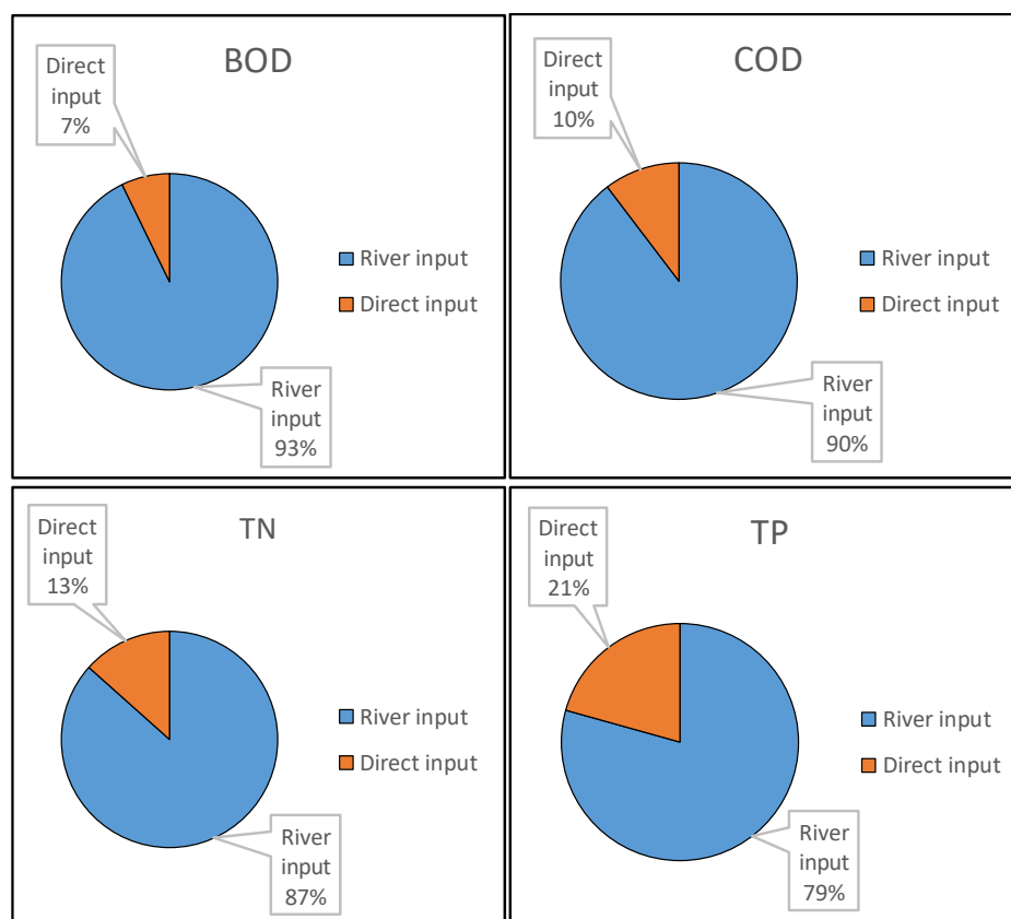
Figure 47. The quota of river and direct inputs of contaminants (BOD, COD, TN and TP) within Toyama prefecture in 2012 (Data source: Toyama Prefecture Water Quality Program, published by Toyama Prefecture, 2015)
