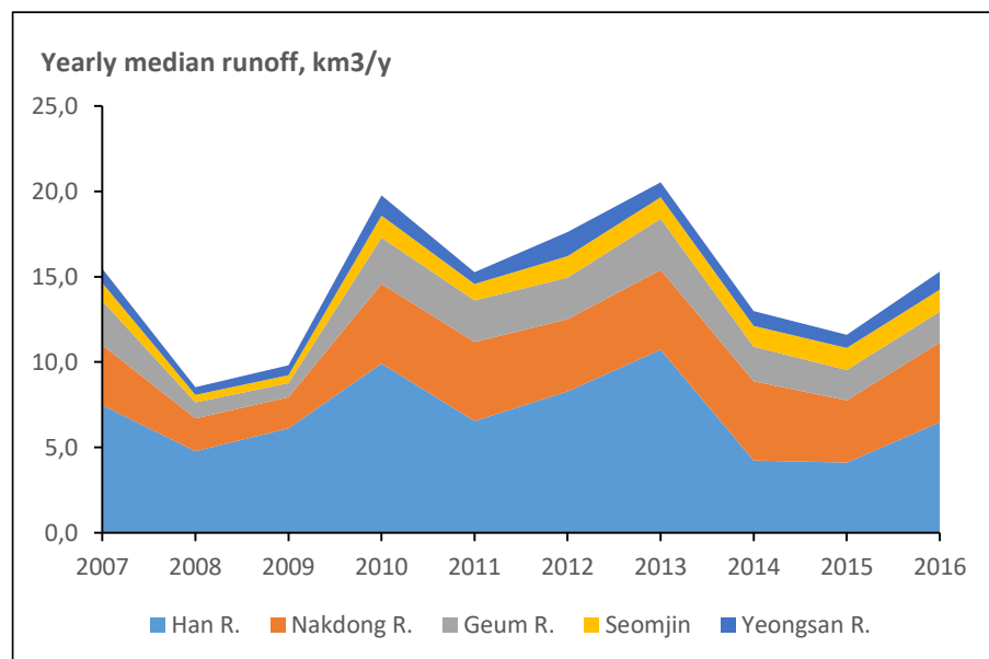
Figure 28. Inter annual variability of the yearly median runoff of the major Korean rivers during last decade (Source: http://www.wamis.go.kr ).
