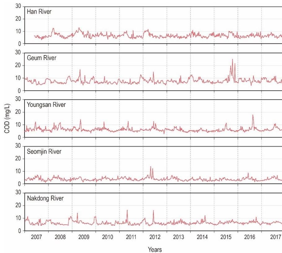
Figure 26. Temporal concentrations of chemical oxygen demand (COD) in five major rivers in Korea from 2007 to 2017.
