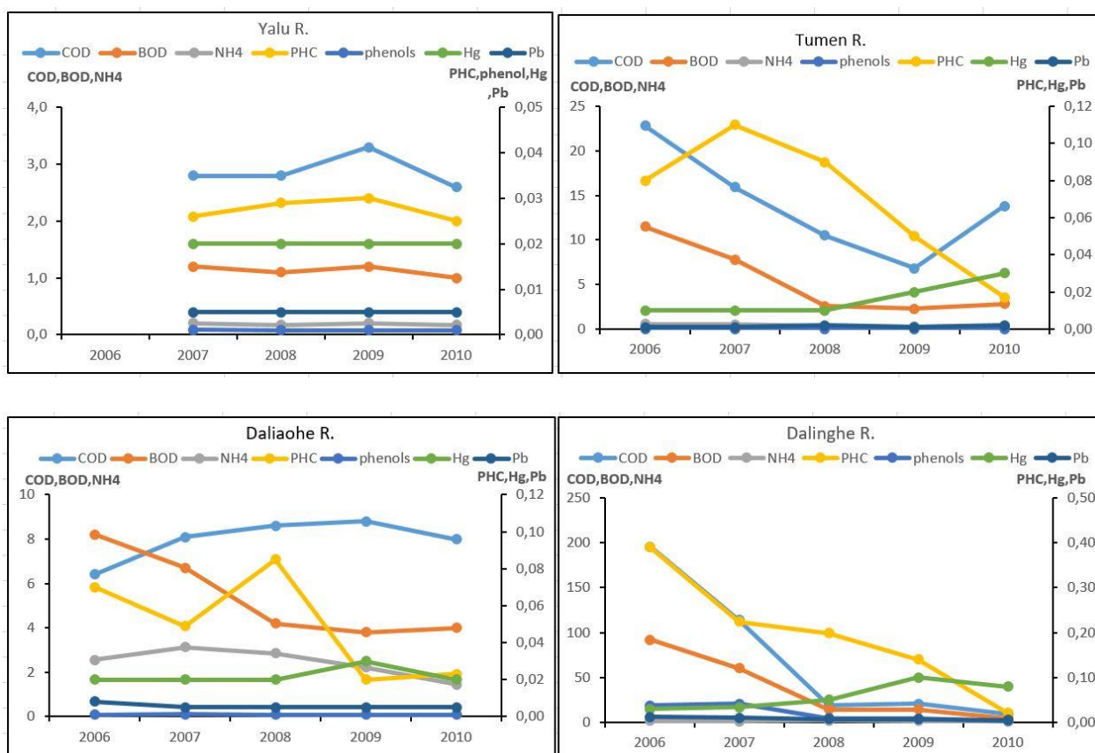
Figure 23. Inter-annual variation of water quality of the typical rivers of northeastern China with different level of pollution.
