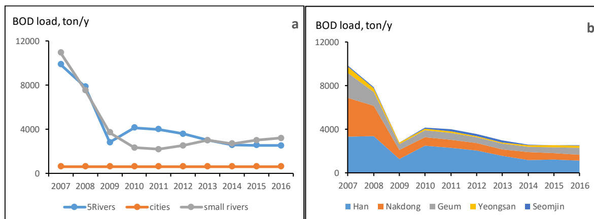
Figure 39. Dynamic of BOD load from different sources (a) and at the watersheds of major Korean rivers during last decade
