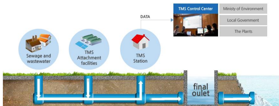
Figure 18. Overview of water TMS ( www.keco.or.kr ).
