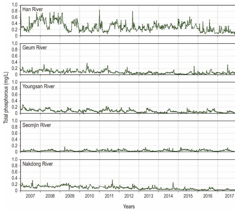
Figure 25. Temporal concentrations of Total Phosphorous (TP) in five major rivers in Korea from 2007 to 2017.
