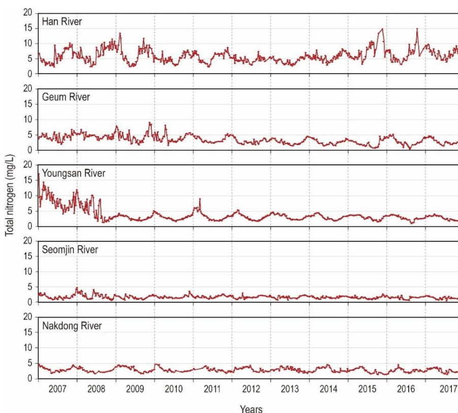
Figure 24. Temporal concentrations of Total Nitrogen (TN) in five major rivers in Korea from 2007 to 2017.
